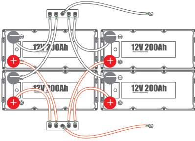
Method 1 (Optimal)
