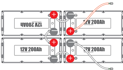
Method 1
