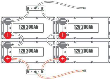
Method 1 (Optimal)
